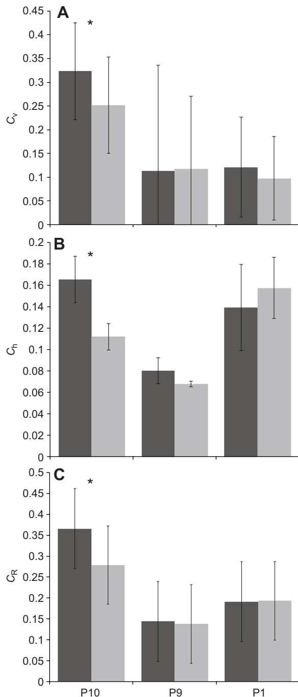
Fig. 7. Mean coefficients of aerodynamic force production of spinning rock pigeon ( Columba livia ) feathers at two velocities. Dark bars represent coefficients of force for feathers spun at average angular velocity (38.1 rad s -1 ) and light bars represent coefficients of force for feathers spun at the angular velocity at which P10 begins to flutter (i.e. U^* ; between 53.9 and 60.3 rad s -1 ). (A) Vertical force coefficient ( C_v ), (B) horizontal force coefficient ( C_h ) and (C) resultant coefficient ( C_R ), which is a vector-sum of C_v + C_h . P10 displayed a significant decrease in all coefficients of force when spun at higher angular velocities. All other feathers showed no significant change. Asterisks indicate statistically significant differences among means ( P < 0.05 ). N = 5 for each bar; data are means \pm s.d.
