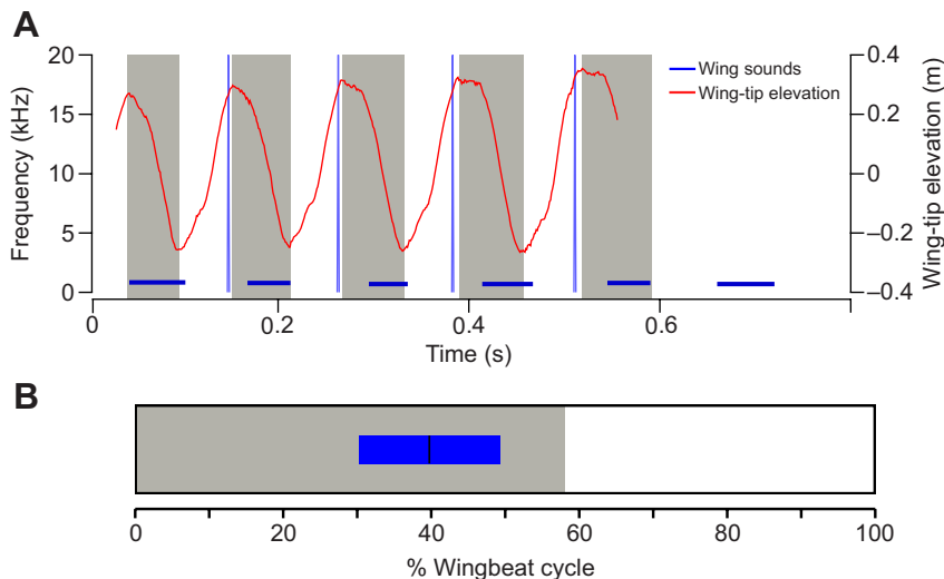
Fig. 6. Synchronized audio and high-speed video recordings of take-off flights reveal that tonal components of wing sounds occur late in downstroke. (A) A single take-off event of synchronized kinematic and acoustic data shows that broadband, atonal claps (vertical blue lines) occur at the top of upstroke, when the wing-tip is highest above the body (red line), and occurs at the end of the first four wingbeats only. Tonal elements (horizontal blue lines) appear to occur late in downstroke and have a peak fundamental frequency of around 700 Hz with up to four harmonics (removed for clarity). Tonal elements occur during the first six downstrokes during this take-off event. Wing-tip elevation data end shortly after the fourth cycle, when the bird flies out of the video frame. (B) Across all video-recorded wingbeats in all birds ( N=20 ), the peak fundamental frequency of the tonal component of wing sounds occurs at 30 \pm 10\% of the wingbeat cycle (or 69 \pm 16\% of each downstroke) during take-off (blue bar). The gray shaded regions in A and B represent the downstroke.
