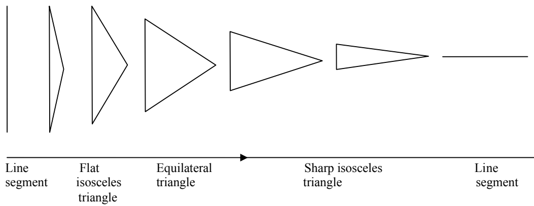
Figure 1. A continuous variation of a triangle
